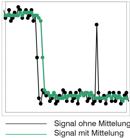
Abb. 59 Median, N = 7
