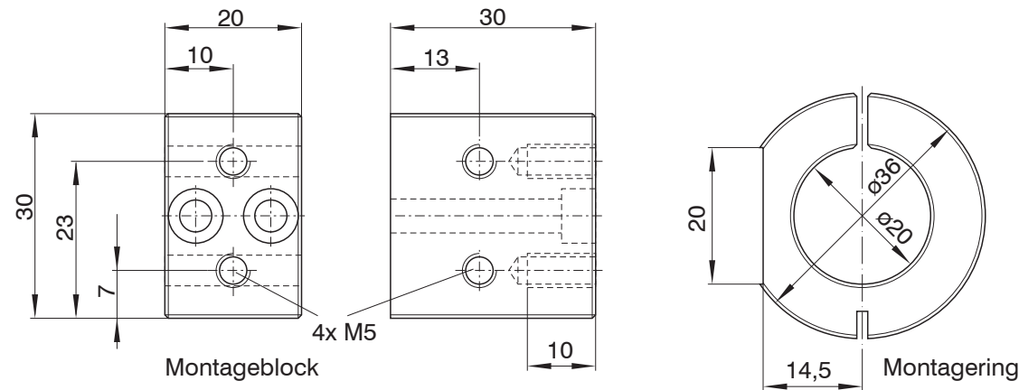
Abb. 29 Montageadapter MA5400-20
