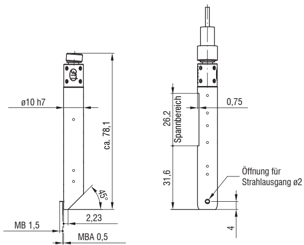
Abb. 23 Abstandssensor IMP-DS0.5/90/VAC
