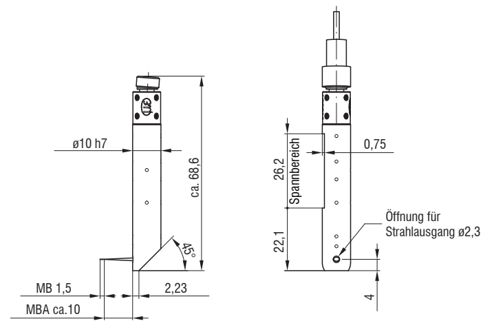
Abb. 24 Abstandssensor IMP-DS10/90/VAC
