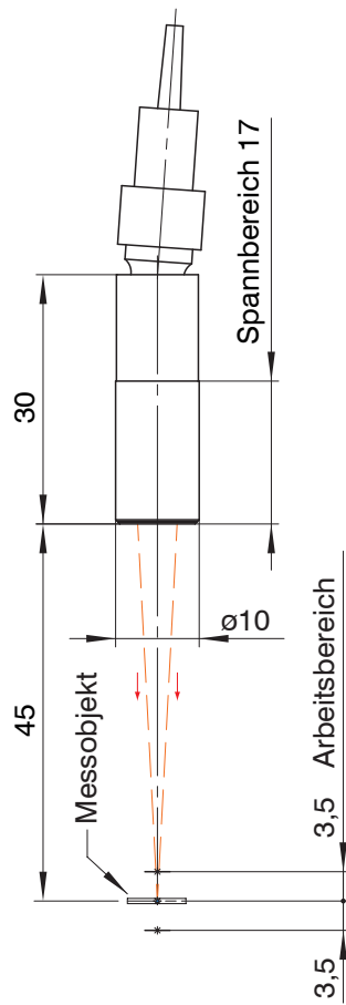
Abb. 26 Dickensensor IMP-TH45
