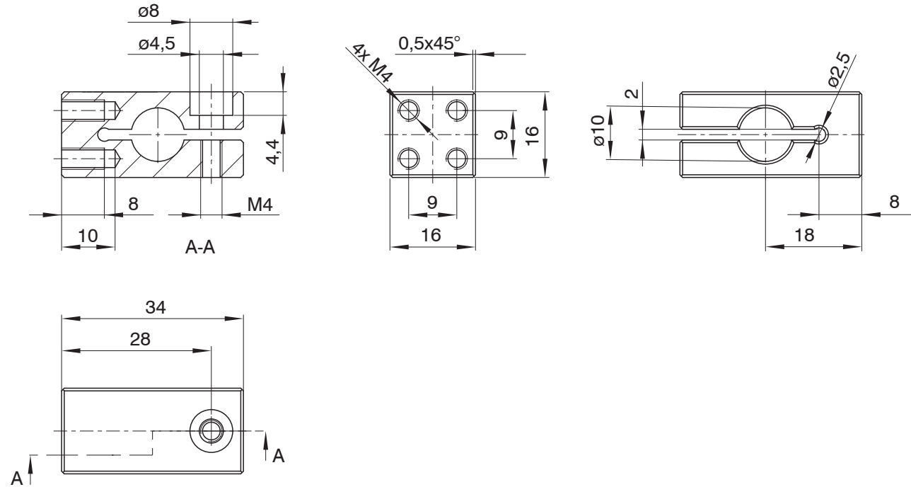
Abb. 28 Montageadapter MA5400-10
