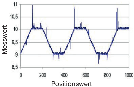
Abb. 60 Profil, Original
