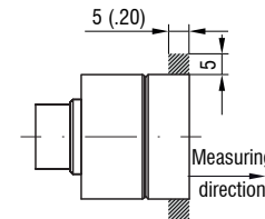
Fig. 5 Dimensional drawing of sensor
