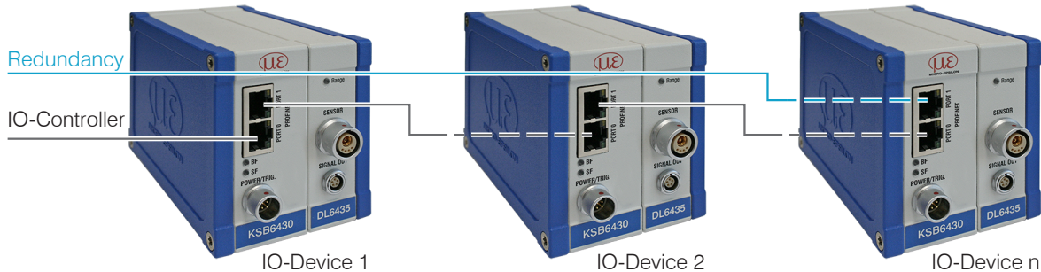
Fig. 12 Cabling in the PROFINET IO network
