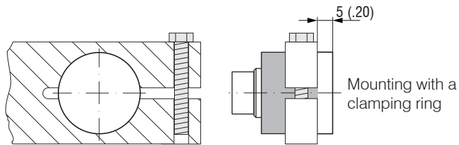
Fig. 7 Circumferential clamping
