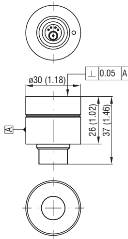
Fig. 5 Dimensional drawing of sensor
