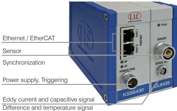
Fig. 4 Controller ports
