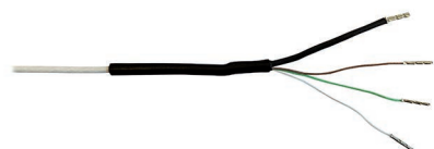
Fig. 7 Assembled sensor cable
