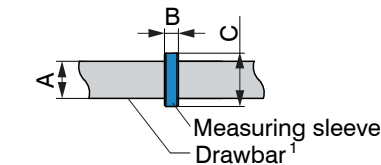
Fig. 5 Drawbar with sensor
